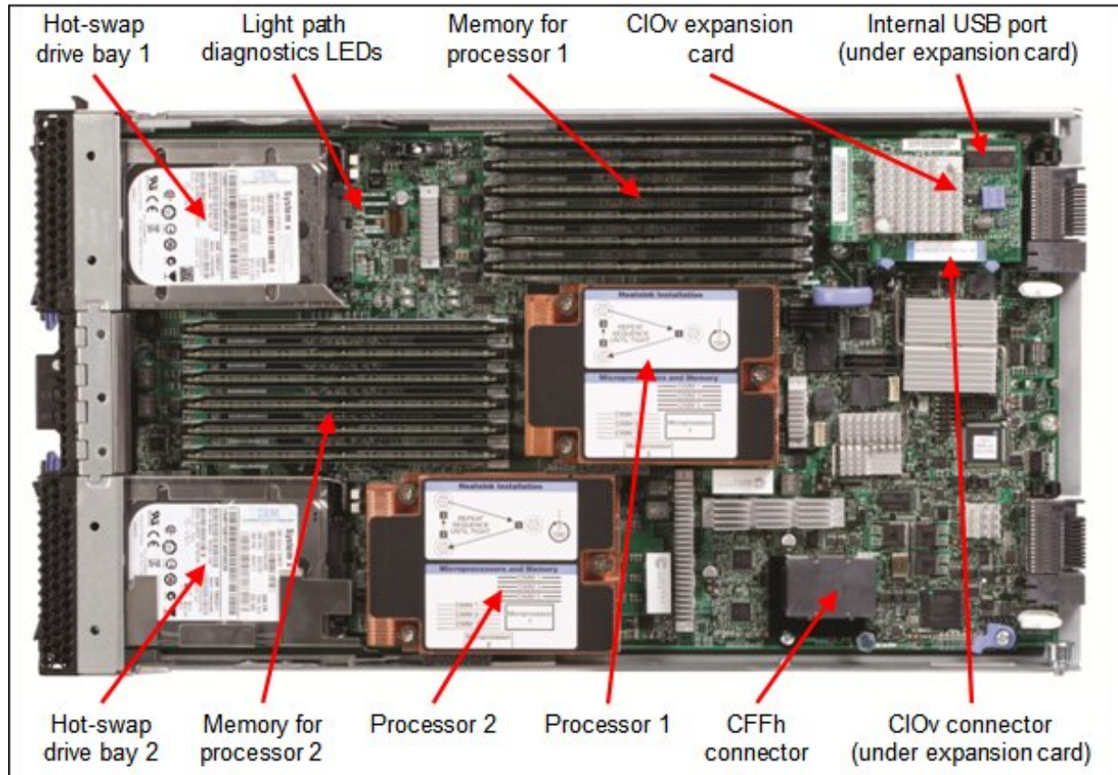
Figure 3. Top view of the IBM BladeCenter HS23E
