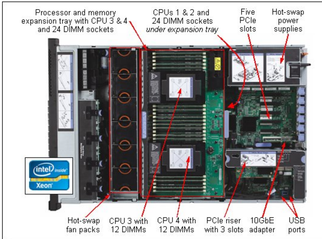
Figure 4. Inside view of the System x3750 M4
