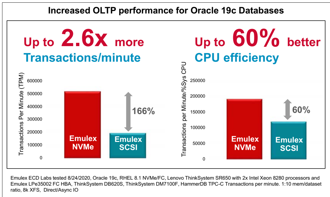
Figure 13 Oracle 19c database
