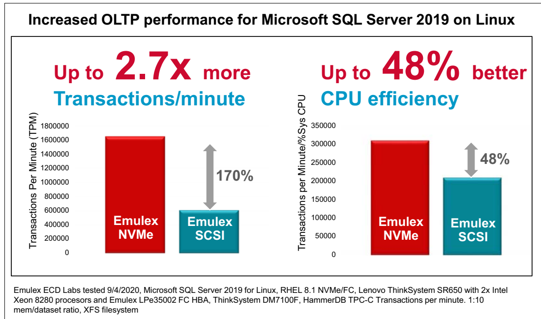
Figure 14 Microsoft SQL Server 2019 database
