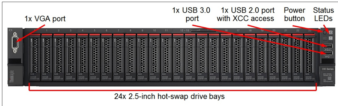
Figure 2. ThinkAgile HX7520 Appliance for SAP HANA front view
