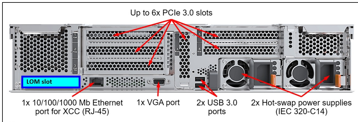
Figure 3. ThinkAgile HX7520 Appliance for SAP HANA rear view
